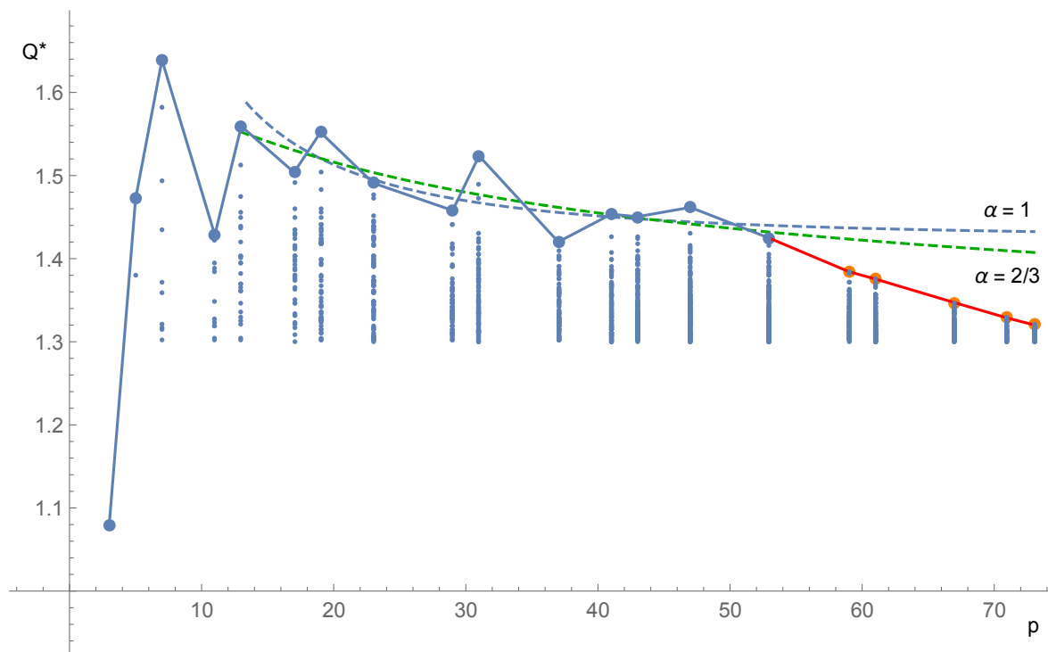
Figure 1: The found triples with Q^*(X, Y, Z) > 1.3 , highlighting the champions, and regression lines for the champions
